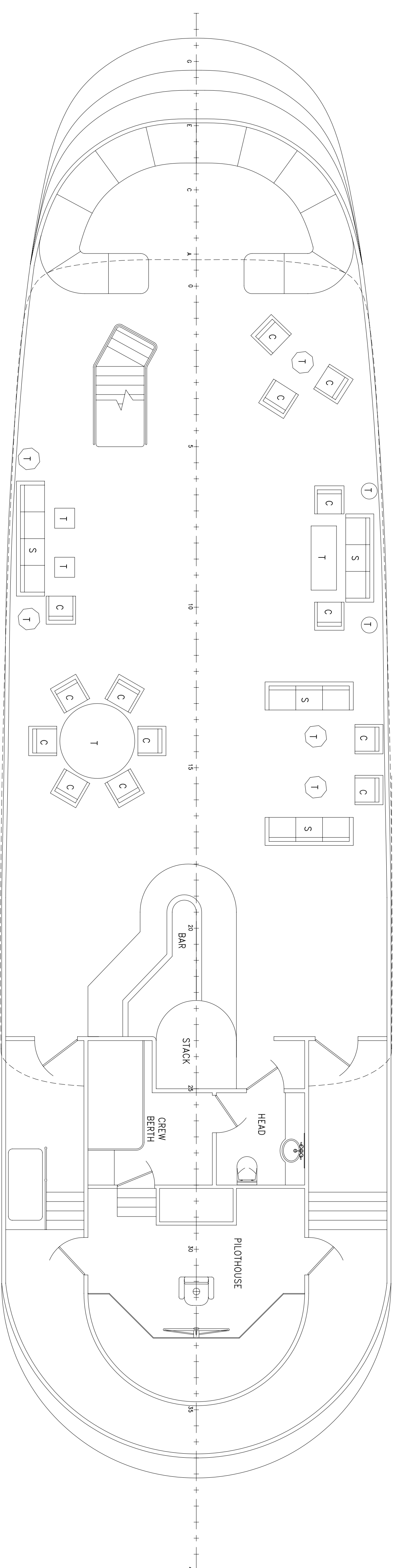
PLAN - SUN DECK & PILOTHOUSE
